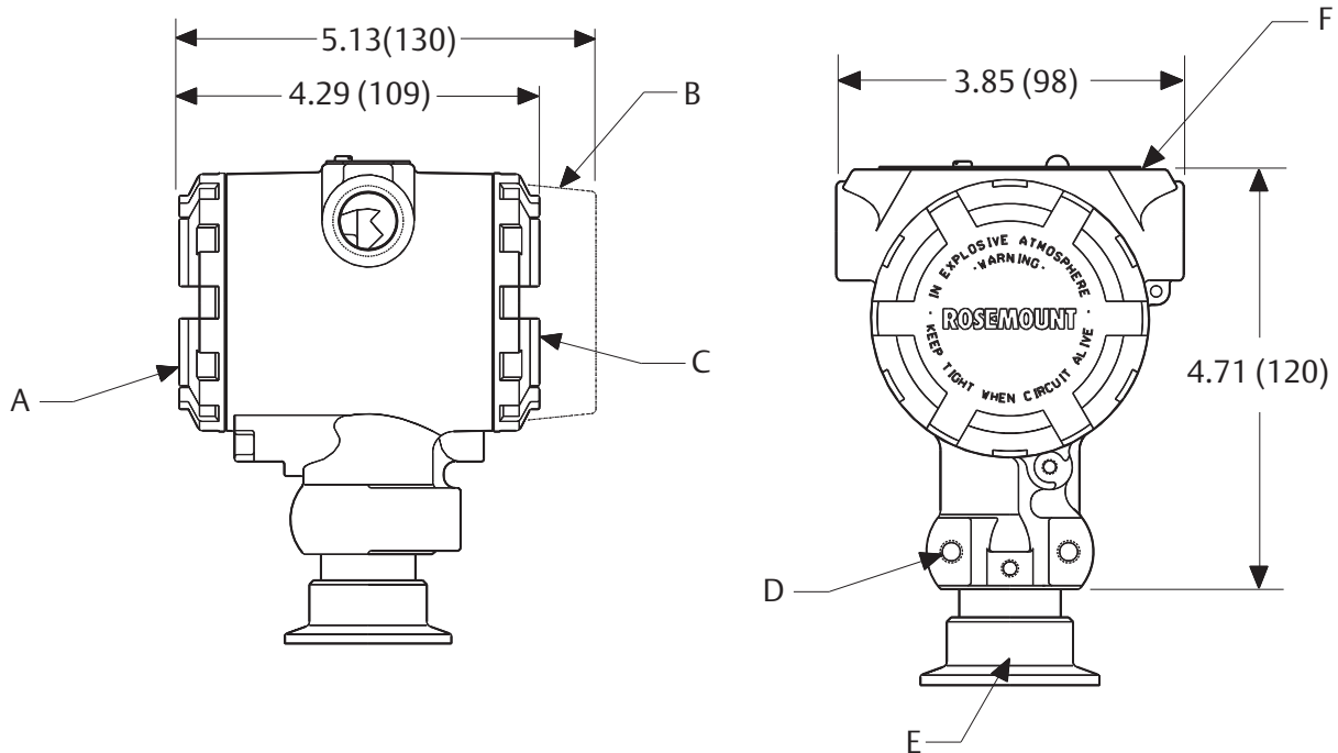
Figure 1. Rosemount 2090F
